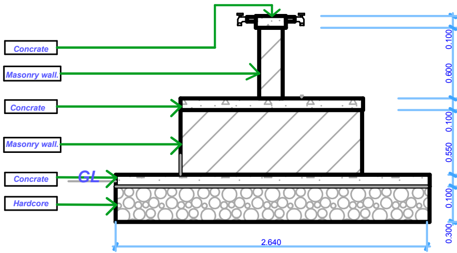
Section S-01
